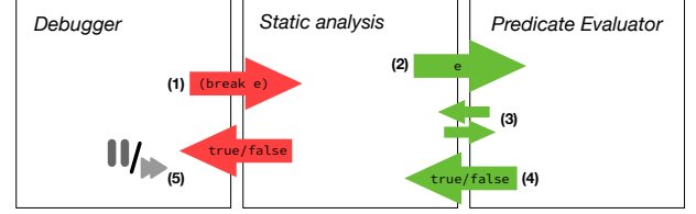
Figure 2. Interactions between the debugger and the meta-predicate evaluator.
